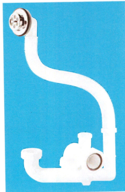
1 1/2" x 50mm Water Seal Anti-Syphon (Silentrap) with flexible overflow tube and CP overflow grating
