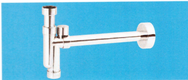
1 1/4" x 50mm Water Seal Plastic Adjustable Inlet Tubular Anti-Syphon Trap (Silentrap) with 12" length of 32mm OD CP brass waste pipe and wall flange
