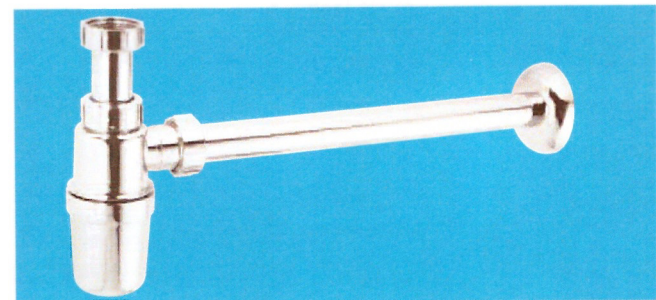
1 1/4" x 75mm Water Seal Brass Adjustable Inlet Bottle Trap with 16" length of 32mm OD CP brass waste pipe and wall flange
