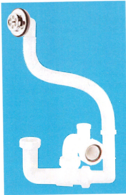
1 1/2" x 75mm Water Seal Anti-Syphon (Silentrap) with flexible overflow tube and CP overflow grating
