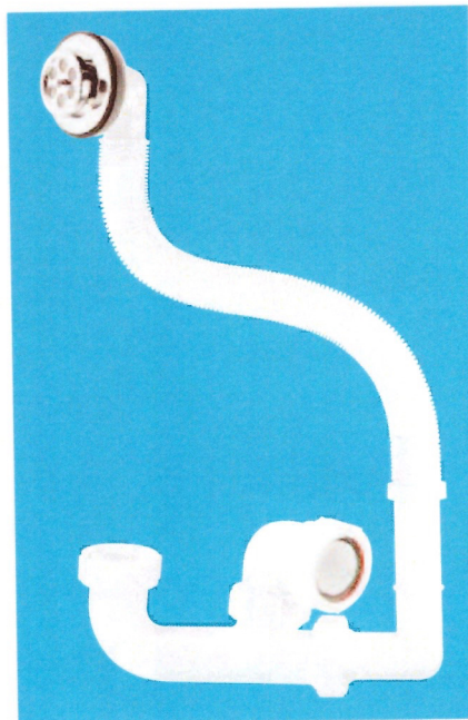
1 1/2" x 50mm Water Seal with flexible overflow tube and CP overflow grating
