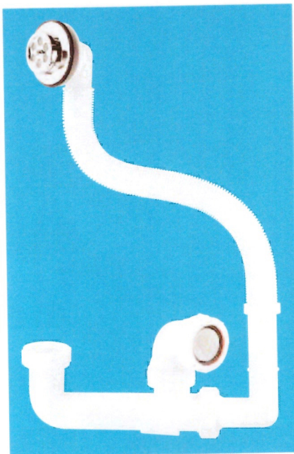
1 1/2" x 60mm Water Seal (Extended Body) with flexible overflow tube and CP overflow grating
