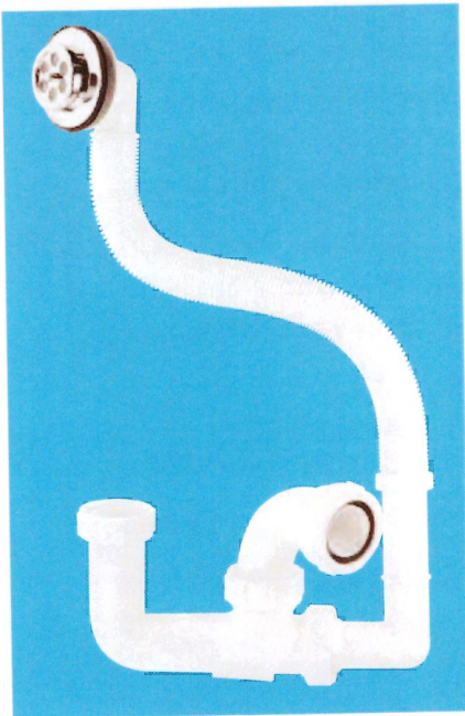
1 1/2" x 75mm Water Seal with flexible overflow tube and CP overflow grating
