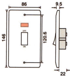
CMA203, CMA503
