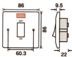
CMA201, CMA501
