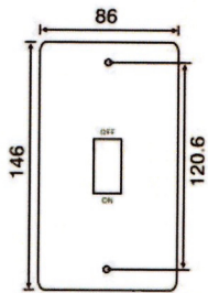
CMA202, CMA502
